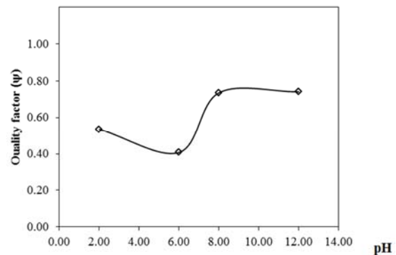
Figure 1. Variation of the quality factor with the pH value of the waste water containing detergent ( B = 0.28 T, d = 6.28 mm, \delta = 2\mu\text{m} , V_f = 0.15\text{m/s} , %1 detergent (w/v), L = 0.1\text{m} ).
