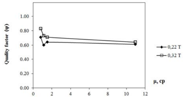
Figure 4. Variation of the quality factor with the viscosity of waste water ( V_f=0.15 m/s, \delta=2\mu\text{m} , d=6.28 mm, L=0.1 m, C_i=50 ppm).
