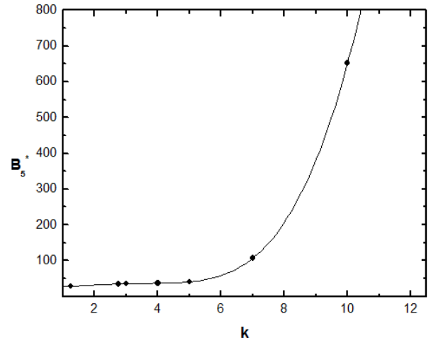
Figure 4. Reduced fifth virial coefficient for prolate spheroids versus elongation, k . The solid and dotted curves are the present work and data obtained by numerical method [31].
